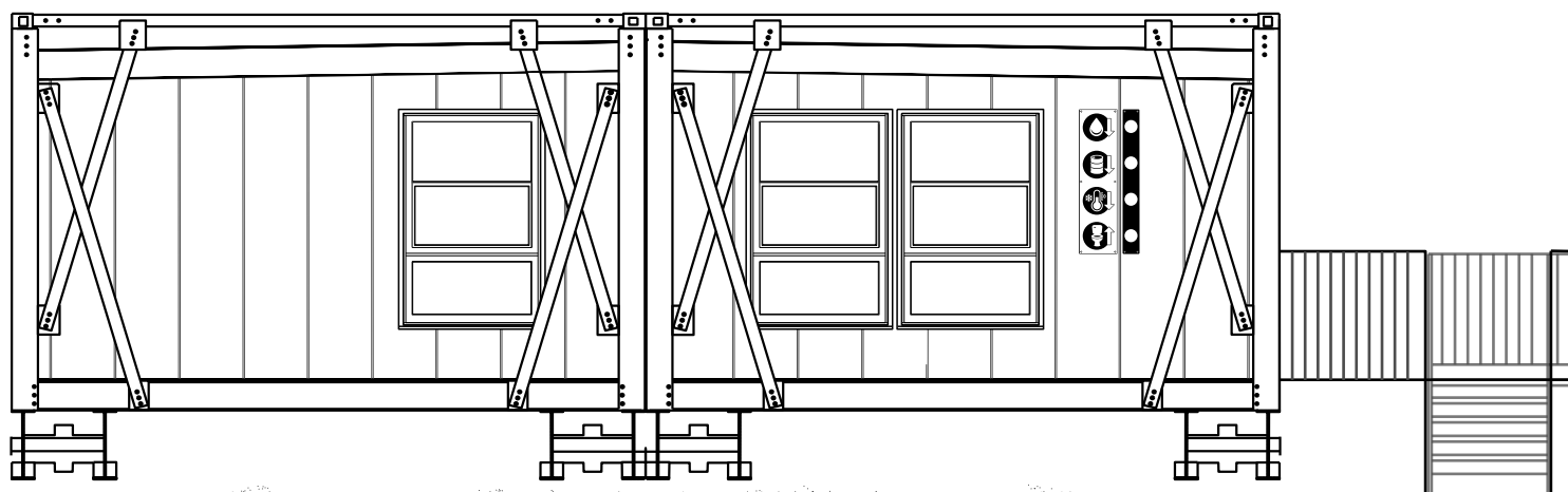
FAÇADE
