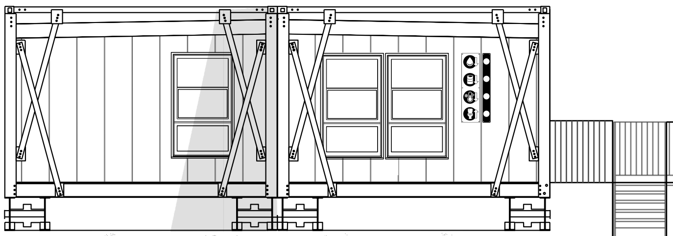
FAÇADE
