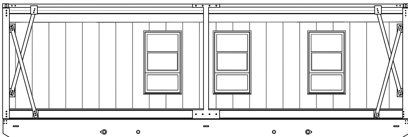
FAÇADE
