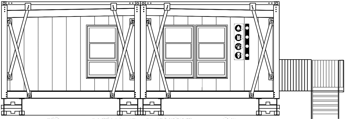
FACADE
